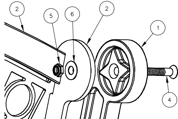
BOLTING DETAIL
