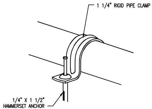
ANCHORING DETAIL
